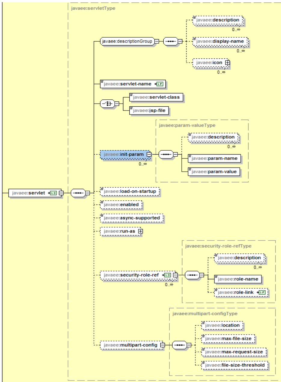
FIGURE 14-5 servlet Element Structure
