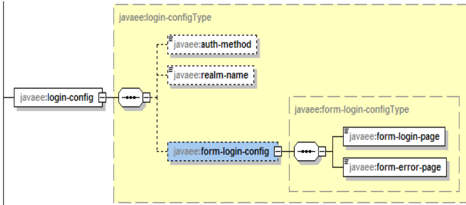
FIGURE 14-13 login-config Element Structure
